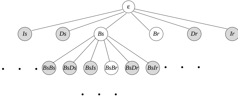
Figure 3: The set of views for the example of Section 2.
