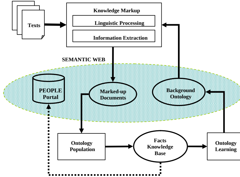
Fig. 1. ONTOTEK Information flow.
