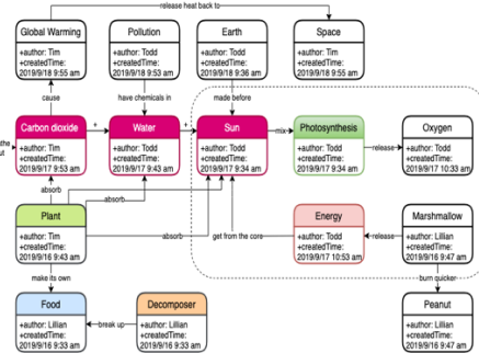
Fig. 3. Collective Temporal Graph.
