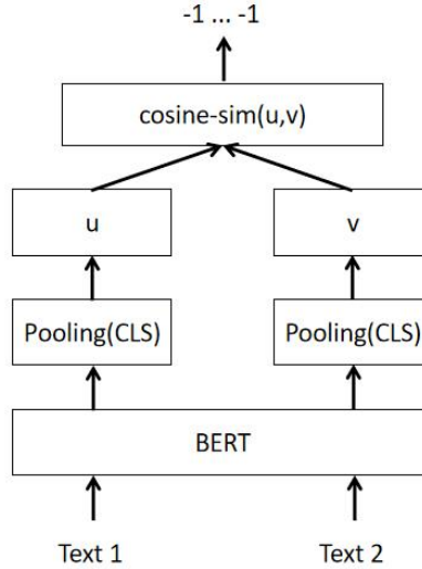
Figure 1: Architecture diagram for our model.
