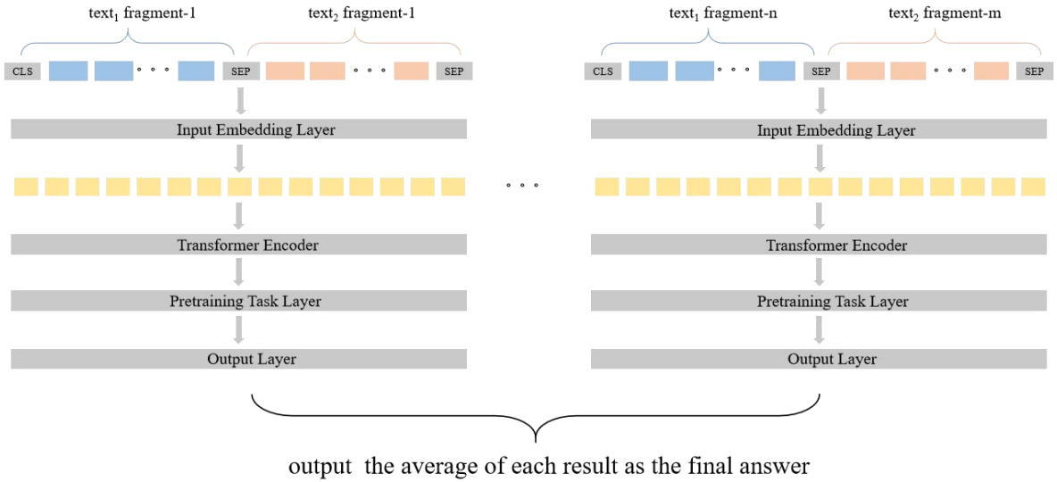
Figure 2: Model training process
